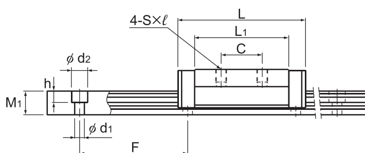
Models SHW17CRM and SHW21CR
