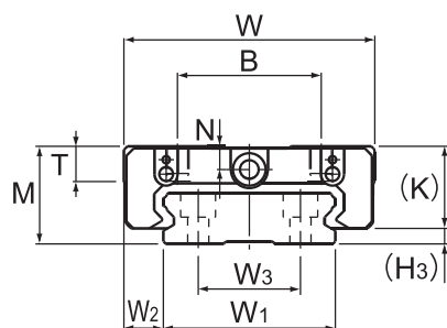
Models SHW12CRM, SHW12HRM and SHW14CRM
