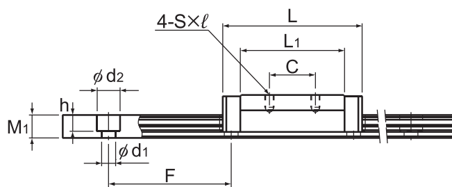
Models SHW12CRM, SHW12HRM and SHW14CRM
