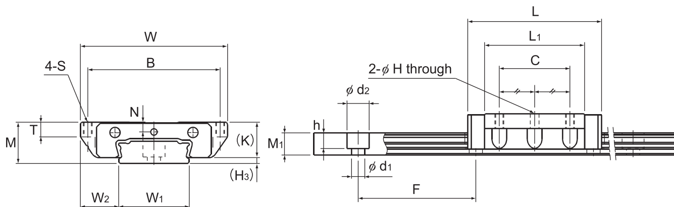
Models SHW12CAM and SHW14CAM
