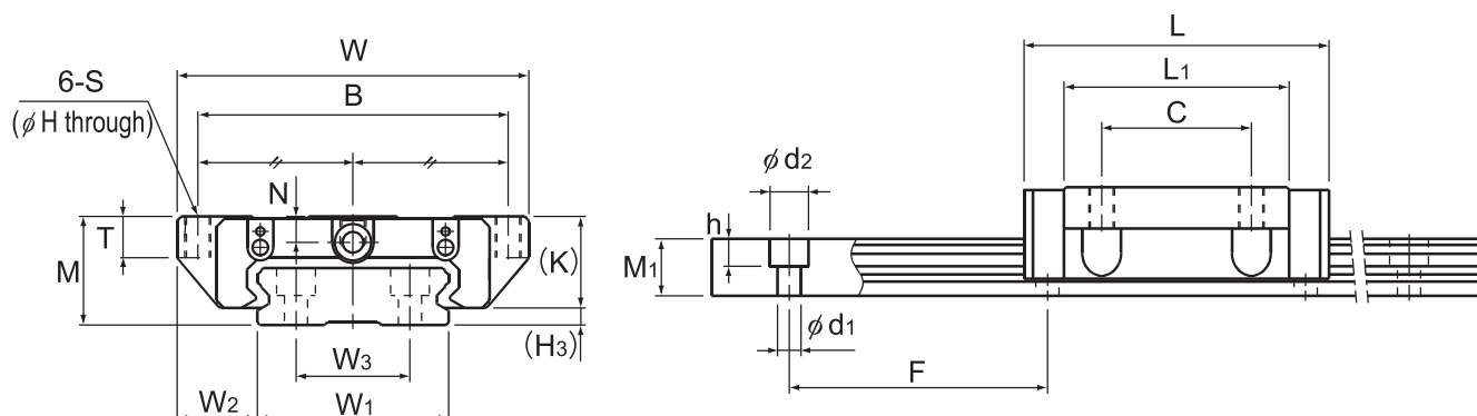
Models SHW17CAM and SHW21 to 50CA
