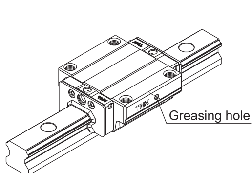
Type with a Greasing Hole Drilled on the Side Surface
